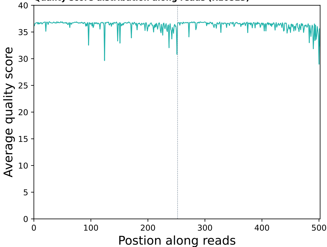
Quality score distribution along reads (R10523)
